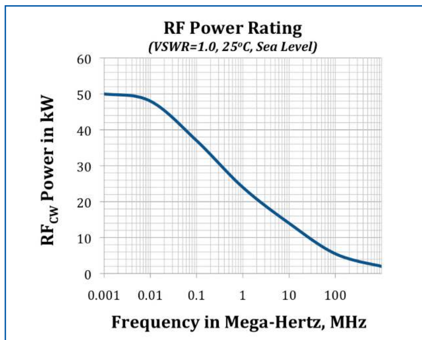
Figure 3: RF Power Rating of the PTR 7AF7AFxxK
