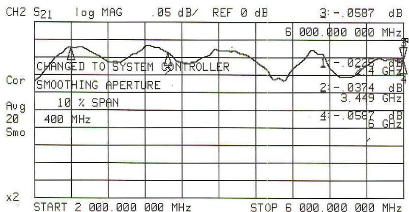
Typical VSWR and Insertion Loss
